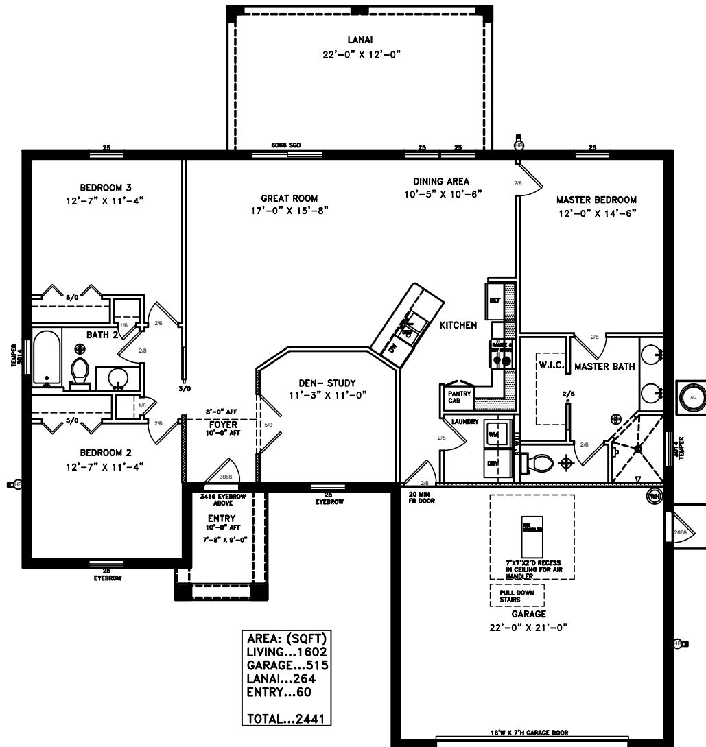
THE DANE (54'-0"W X 61'-8"D) © COPYRIGHT TRINITY DRAFTING LLC
