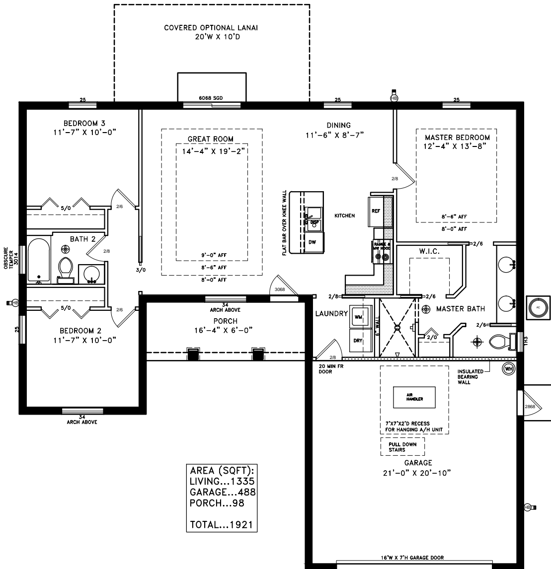
THE NAPLES (51'-8"W X 48'-0"D) © COPYRIGHT TRINITY DRAFTING LLC
