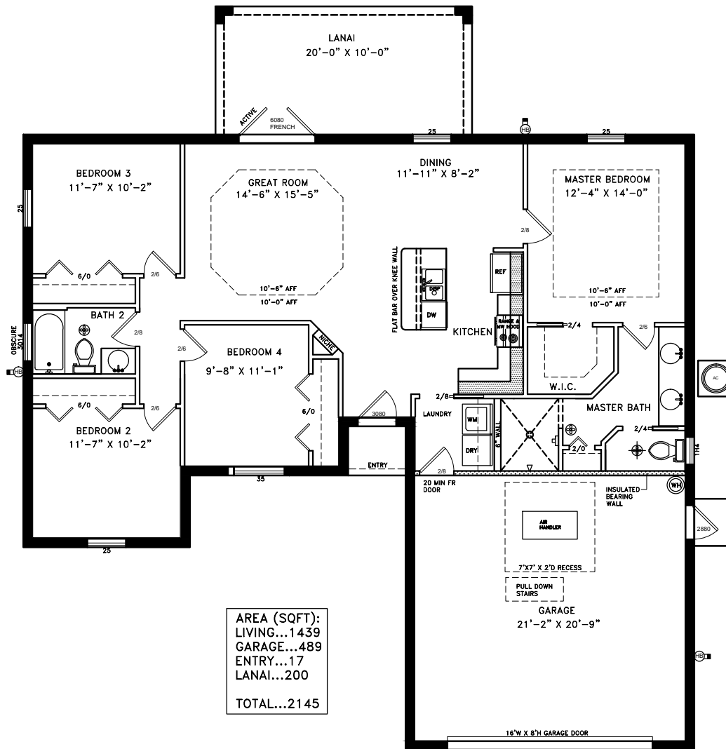
THE REDINGTON 4 (52'-4"W X 58'-0"D) © COPYRIGHT TRINITY DRAFTING LLC
